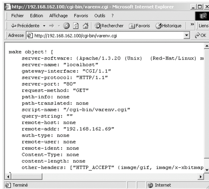
Figure 4-5. CGI environment variables.
